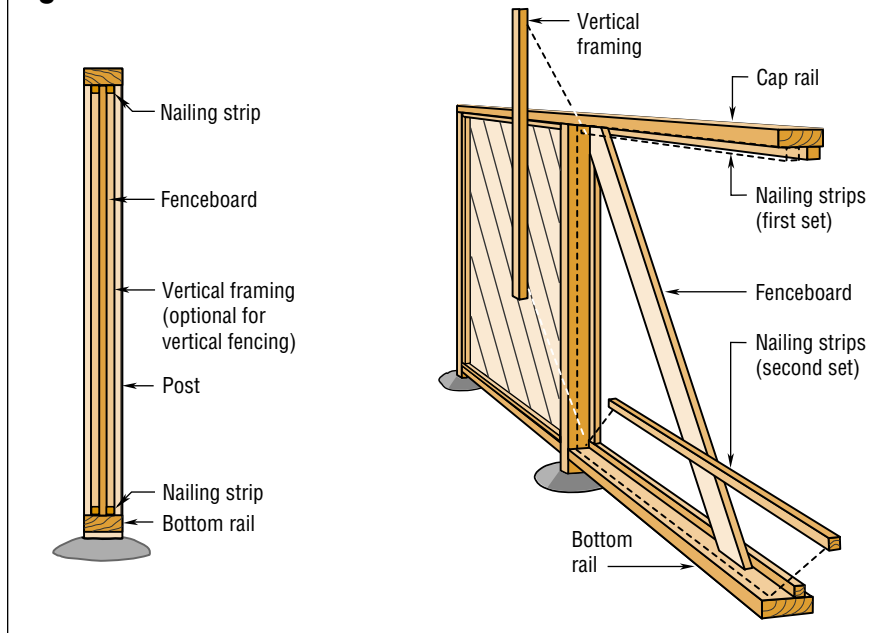
Fig. 9: INSET FENCING
