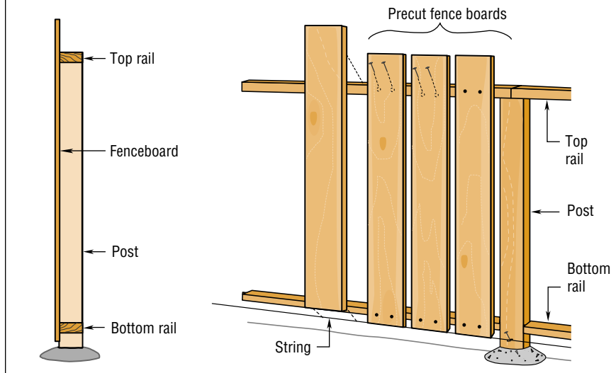
FIG. 8: NAIL-ON FENCING
